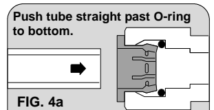
FIG. 4 Quick Connect/Push-in Connector
