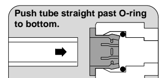
FIG. 4 Quick Connect / Push-in Connector
