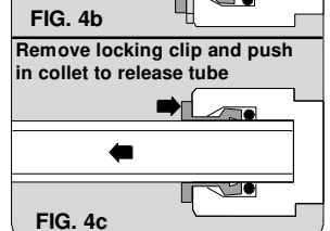
FIG. 4 Quick Connect / Push-in Connector
