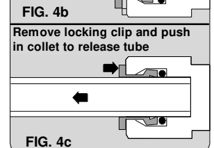
FIG. 4 Quick Connect / Push-in Connector
